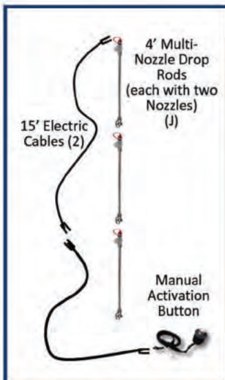
MULTI-ROD SYSTEM
